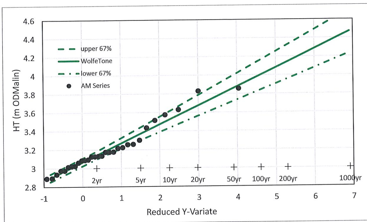
Figure 3-12 Tidal Flooding H – T with 67-percentile upper and lower confidence Intervals based on EV1 analysis of the Wolfe Tone Gauge
