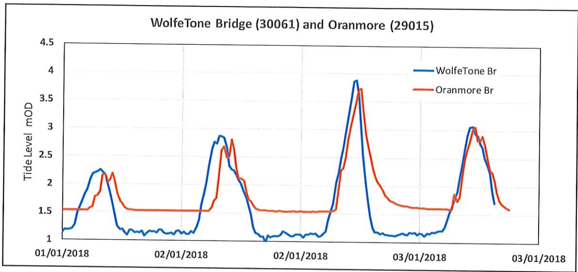
Figure 3-6 Tidal Flood Event recorded at Wolfe Tone Bridge Galway City and Oranmore Bridge on the 2nd of January 2018 (Storm Eleanor)
