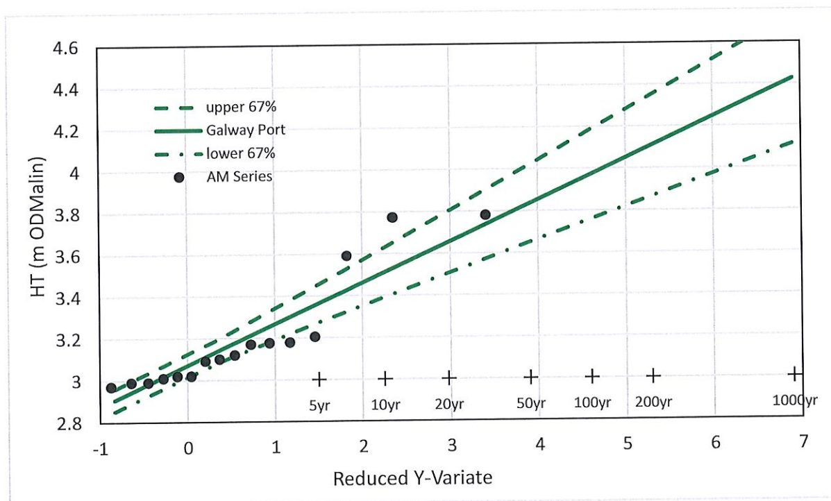
Figure 3-13 Tidal Flooding H – T with 67-percentile upper and lower confidence Intervals based on EV1 analysis of the Galway Docks Gauge
